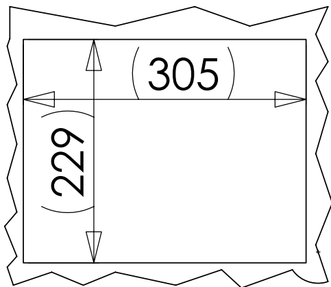
Customer Panel Cut out
